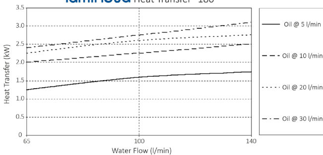
laminova Heat Transfer- 180
