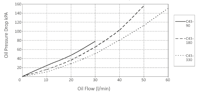
laminova Oil Pressure Drop
