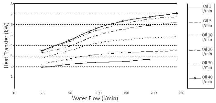
laminova Heat Transfer- 180
