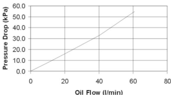
OIL PRESSURE DROP ECD54-329
