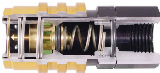
Internal view of a standard Jiffy-tite socket
