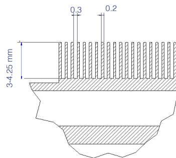
Cross section of a core showing height of fins, distances between them and their thickness in mm.
