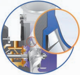
Compressor wheel with extended tip technology
